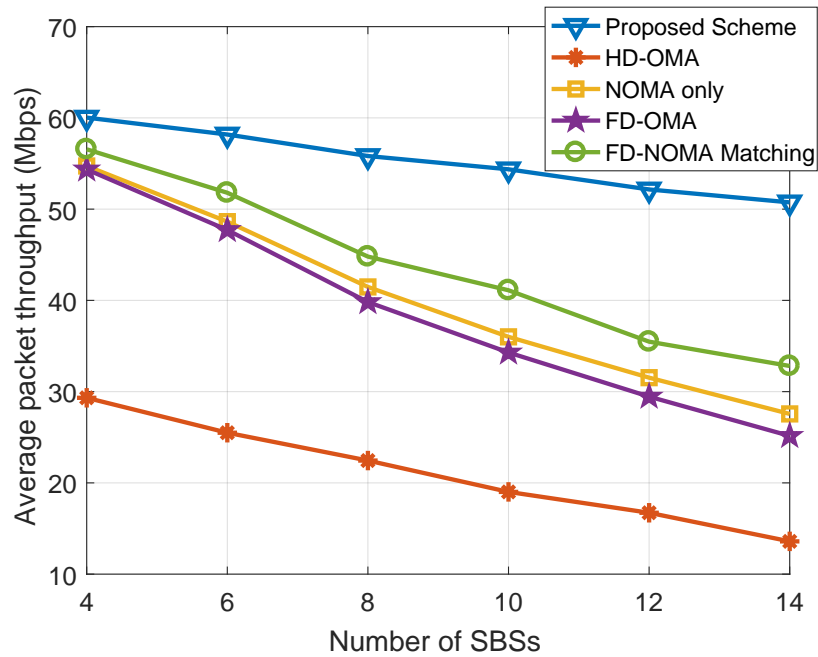
Figure 7. Average packet throughput performance for different schemes as the network density increases for an average of 10 UEs per SBS and a mean traffic intensity of 3 Mbps per user.
