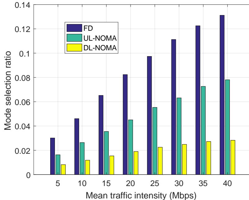
Figure 4. FD and NOMA mode selection ratios at different traffic intensity levels, for a network of 10 SBSs and an average of 10 UEs per SBS. Remaining transmissions are in HD-OMA mode.
