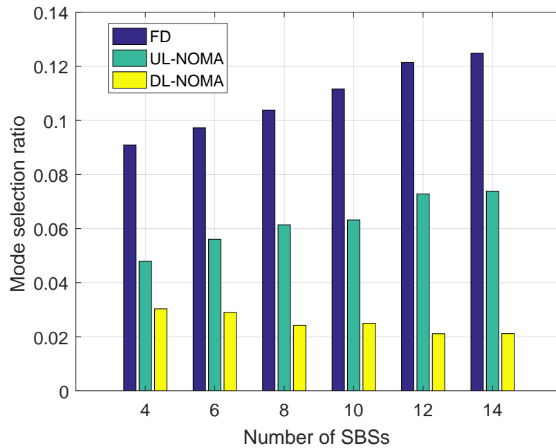
Figure 8. FD and NOMA mode selection ratios as the network density increases for an average of 10 UEs per SBS and a mean traffic intensity of 3 Mbps per user. Remaining transmissions are in HD-OMA mode.
