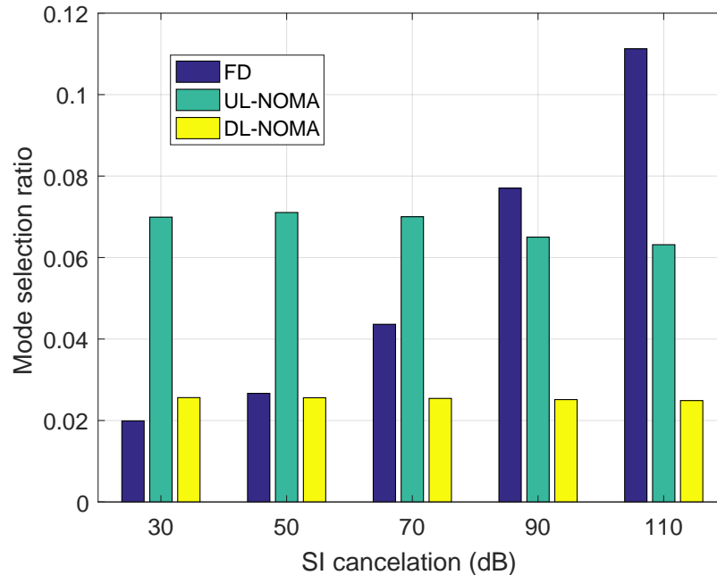
Figure 10. FD and NOMA mode selection ratios at different SBS SI cancellation capability levels, for a network of 10 SBSs, an average of 10 UEs per SBS, and a mean traffic intensity rate of 3 Mbps per user. Remaining transmissions are in HD-OMA mode.
