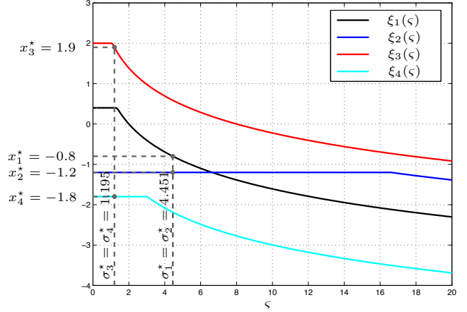
Fig. 1. Graphical illustration of the solutions x_n^* . The intersection of \xi_n(\varsigma) with the vertical dashed line at \varsigma = \sigma_n^* yields x_n^* .
