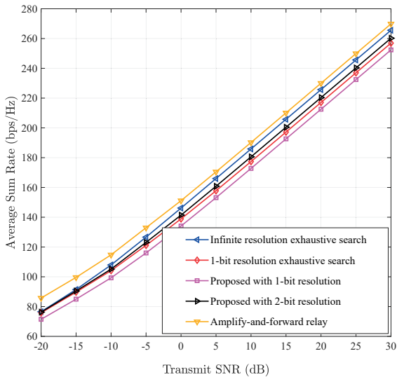
Figure 5. Achievable sum rate vs the transmit SNR for K = 16 , M = 12 , N = 32 , and R_{\min,k} = \log_2(1 + \frac{\text{SNR}}{2K}) bps/Hz \forall k = 1, 2, \dots, 16 .
