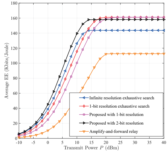
Figure 3. Energy efficiency maximization vs the total BS transmit power P for K = 16 , M = 12 , N = 32 , and R_{\min,k} = 0 bps/Hz \forall k = 1, 2, \dots, 16 .
