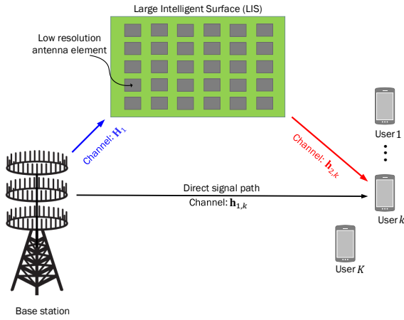
Figure 1. The considered LIS-assisted multi-user MISO system comprising of a M -antenna base station simultaneously serving in the downlink K single-antenna users. LIS is assumed to be attached to a surrounding building's facade, and the transmit signal propagates to the users both directly from the base station and via LIS with reconfigurable behavior.
